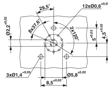
Drilling diagram
